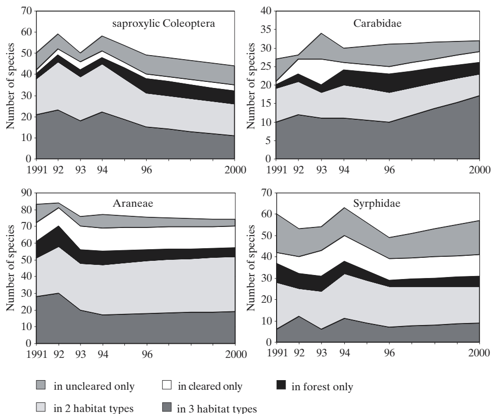
Fig. 2. Development of species numbers in four taxonomic groups at the site in Schwanden. Numbers are split up into species occurring in one treatment or the control only, in two habitat types (cleared and uncleared) or all three habitat types. Species numbers for the years 1995 and 1997 to 1999 are linear extrapolations of the adjacent years (1994, 1996, 2000, respectively).
