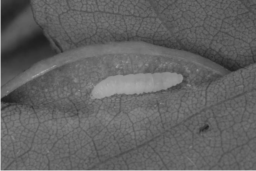
Fig. 2. Opened gall with larva of Obolodiplosis robiniae .
