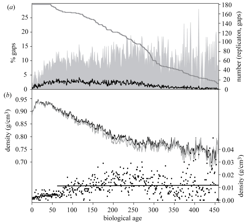
Figure S3. Age-effect in LBM outbreak detection. (a) Larch sample replication (grey curve), number of gaps (black curve), and percent gaps (grey shading), all aligned by biological tree age. Gaps represent LBM-affected tree-rings that were removed from the MXD data. The percent record represents the number of gaps related to the total number of samples for each ring-age (1-460). (b) Mean original (grey) and gap-filled (black) MXD curves after aligning the data by biological age, with sample replication as in (a). Since the gap-filling procedure includes the substitution of LBM-affected (low density) with non-affected (higher density) tree-rings, the gap-filled series shows generally higher values than the original curve. The scatter plot at the bottom of the figure shows the annual differences between gap-filled and original MXD records, and the linear models fit to difference data <63 and >62 years.
