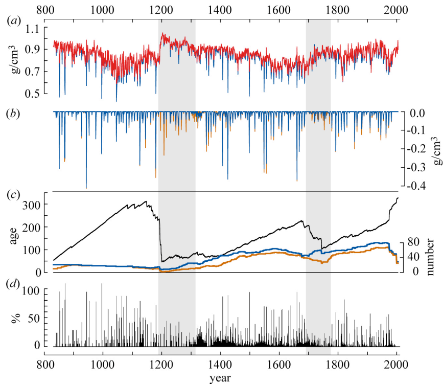
Figure S1. MXD chronology and LBM outbreak detection. (a) Original (blue) and gap-filled (red) MXD records combining data from 180 larch samples. (b) Difference series (blue) between the gap-filled and original data, and the age-effect corrected version of this record (orange). The correction was accomplished by excluding tree-rings younger than 63 years from the data (see figure S3). Values less than -0.005 \text{ g/cm}^3 are shown. (c) Mean age curve of the MXD data (black) shown in (a), and sample replication of the gap-filled (blue) and age-effect corrected (orange) data. (d) Percentage of tree-rings affected by LBM outbreaks. These rings were removed from the data, and re-estimated using data from unaffected rings. The resulting record is shown in (a, red curve). Grey bars indicate low LBM intensity and low mean biological age periods in the 12th and 17th centuries.
