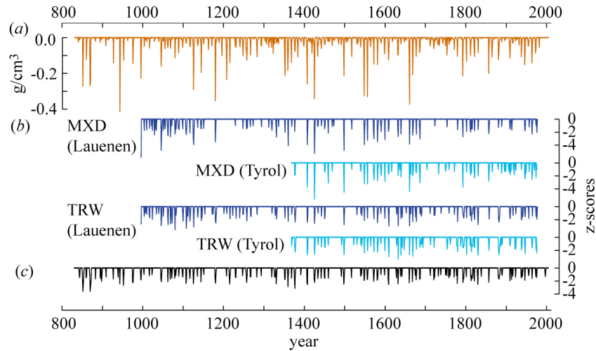
Figure S4. LBM outbreak reconstruction and validation. (a) Age-corrected LBM reconstruction as shown in figure S1b. (b) Difference records between larch (MXD and TRW) data and the non-host fir/spruce chronologies from Lauenen and Tyrol. (c) Combined larch MXD and lag-1 TRW record. For the lagged LBM response in the TRW data see figure S5. MXD and TRW data were detrended using flexible cubic spline filters before combination to emphasize inter-annual variations. Values exceeding one standard deviation are shown.
