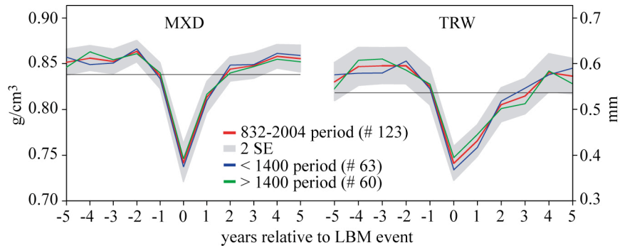
Figure S5. LBM patterns in tree-ring data. Average MXD ( \text{g}/\text{cm}^3 ) and TRW (mm) values centred on the 123 LBM outbreak events (year 0) and 5 years before and after these events (red curve). Grey shadings indicate two standard errors, and horizontal black lines the average MXD ( 0.838 \text{ g}/\text{cm}^3 ) and TRW ( 0.536 \text{ mm} ) values over the 11-year periods displayed here. Blue and green curves are the MXD and TRW patterns calculated using data before and after 1400, respectively. The means for these sub-periods have been adjusted to the average using all data (horizontal lines).
