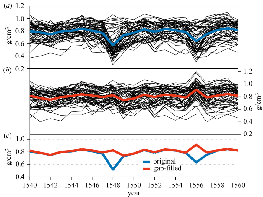
Figure S2. Gap-filling procedure in individual MXD timeseries. (a) Original MXD measurement series including the 1548 and 1556 LBM outbreak years. Each series represents a single larch core sample from which density measurements were computed. (b) Gap-filled MXD measurement series with the LBM effects in 1548 and 1556 removed from the data. (c) Comparison of the original and gap-filled mean records.
