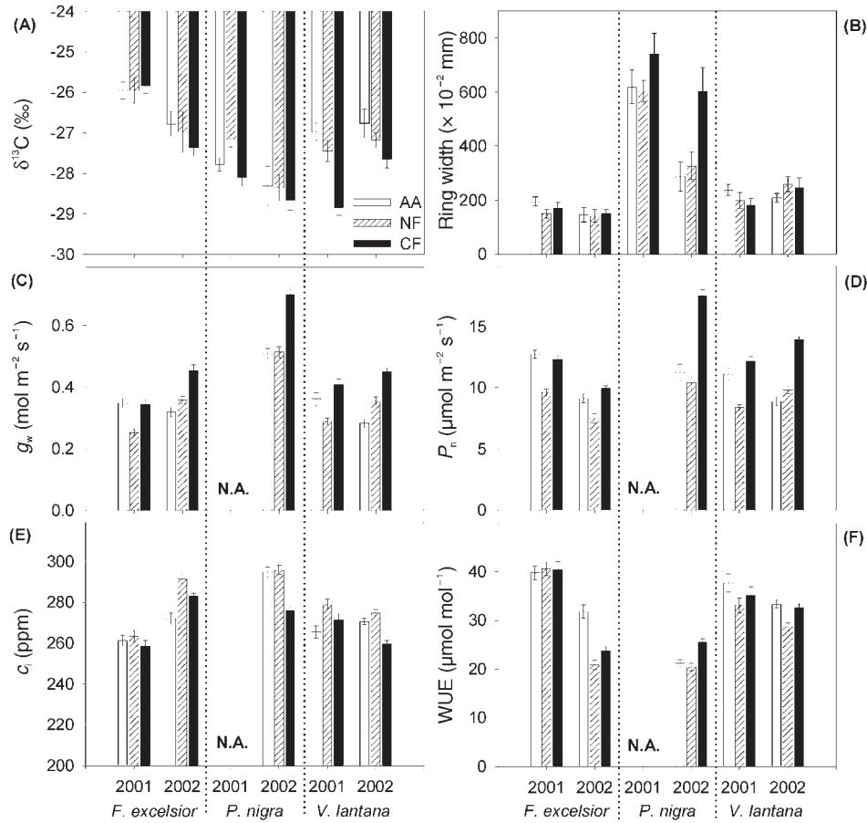
Figure 2. Mean and standard error for stable carbon isotope ratio ( \delta^{13}C ) (A), ring width (B), stomatal conductance to water vapor ( g_w ) (C), net photosynthesis ( P_n ) (D), intercellular CO_2 concentrations ( c_i ) (E) and water-use efficiency (WUE) (F) for Fraxinus excelsior , Populus nigra , and Viburnum lantana grown at the Lattecaldo OTC facility in 2001 and 2002. Gas exchange data for 2002 were recalculated from Novak et al. (2005). Abbreviation: N.A. = not assessed.
