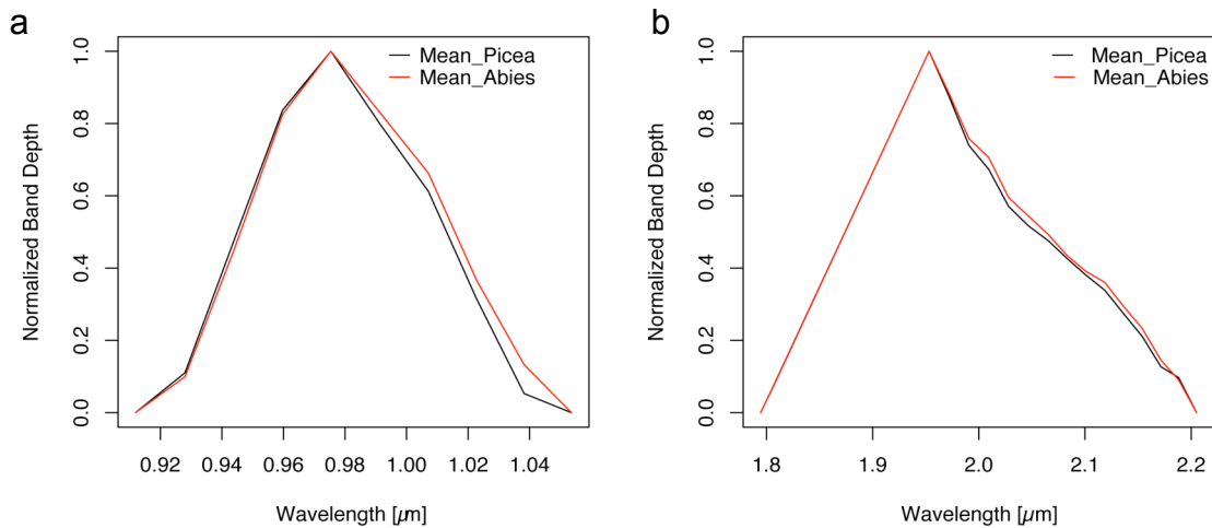
Figure 5: Comparison of normalized band depth of Norway spruce ( Picea abies ) and silver fir ( Abies alba ).
