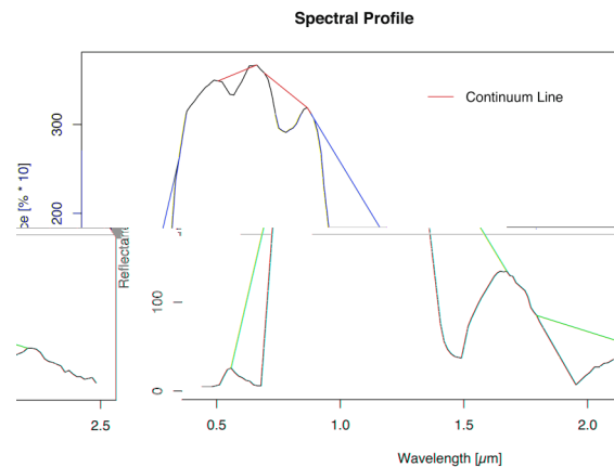
Figure 1: Linear segments used to isolate each nitrogen absorption feature in HyMap reflectance spectrum.
