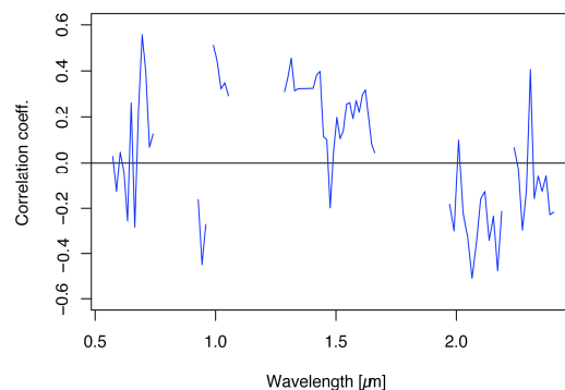
Figure 6: Correlogram on the deciduous spectra of the preselected wavelength ranges using normalized band depths (BNC).
