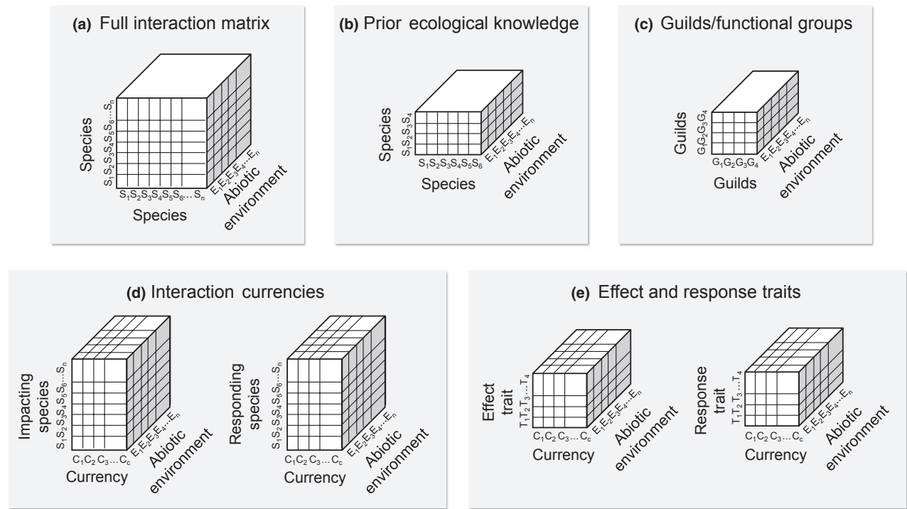
Figure 3 Simplified schematic examples for reducing the complexity and dimensionality when modelling biotic interactions in variable environments. (a) A full interaction matrix with S^2 species quantifies all possible species-by-species interaction coefficients and how they vary as a function of e environmental conditions. (b) Based on a priori ecological knowledge the number of interacting species is smaller than in the full interaction matrix because some species are known not to interact (from field studies, experiments, ecological networks, or natural history information). (c) Aggregating species into groups with similar biological, ecological, physiological or morphological characteristics allows the modelling of guilds, functional groups, or functional types. (d) Modelling species' impacts and responses to interaction currencies (e.g. consumable resources, microclimatic conditions, or pollination and seed dispersal services) can reduce the complexity if the number of interaction currencies is smaller than the number of species. (e) The impacts and responses of species as derived from modelling continuous species' effect and response traits. Here, quantitative traits (rather than species) are used to describe the responses to, and impacts on, specific currencies that mediate interactions.
