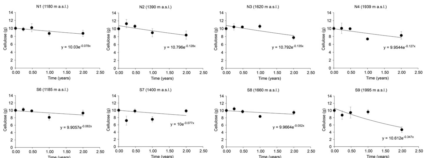
Fig. 4. Amount of cellulose (= concentration \times dry weight of wood block; weight \pm standard error) as a function of time (0–2 years), site (altitude) and exposure (north vs south).
