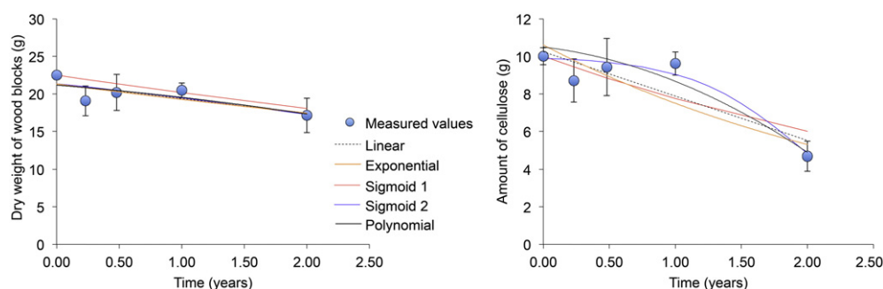
Fig. 6. Comparison of exponential, linear, sigmoid (2 types; sigmoid function 1 (Eq. 4) and sigmoid function 2 (Eq. 5)) and polynomial (2nd order) best-fit decay model for deadwood (dry weight of wood blocks) and amount of cellulose (concentration \times dry weight of wood block) for site S9.
