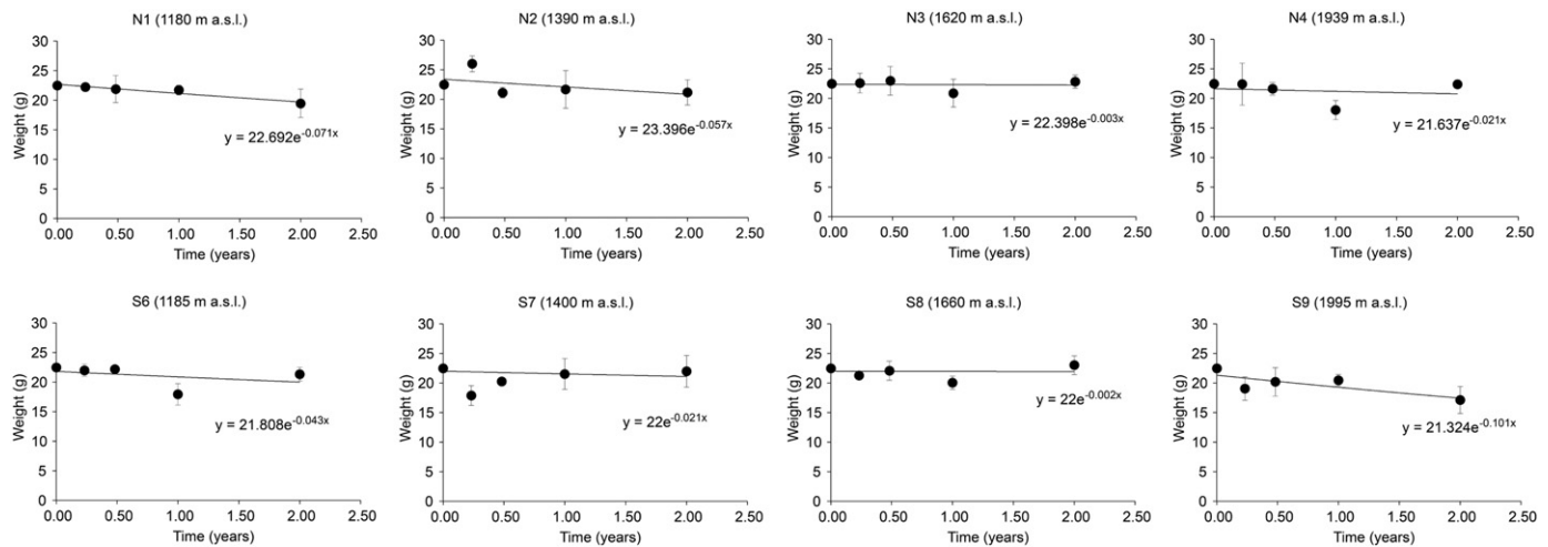
Fig. 3. Weight ( \pm standard error) of the wood blocks (placed into mesocosms) as a function of time (0–2 years), site (altitude) and exposure (north vs south).
