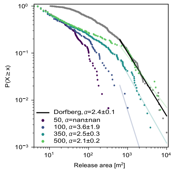
Figure 2: Complementary cumulative distribution function P(X \geq x) \approx x^{-(\alpha-1)} for glide-snow avalanche release areas on Dorfberg and for simulations with varying friction length scales (50, 100, 350, 500). For Dorfberg, the optimal param-
