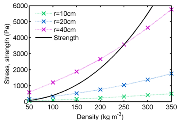
Fig. 2: FE simulation results for the maximal tensile stress at the snow surface in a PST experiment vs slab density for three different crack length ( r = 10, 20, 40 cm). Also shown is the relation for tensile strength reported by Jamieson and Johnston (1990) (Eq. 4).
