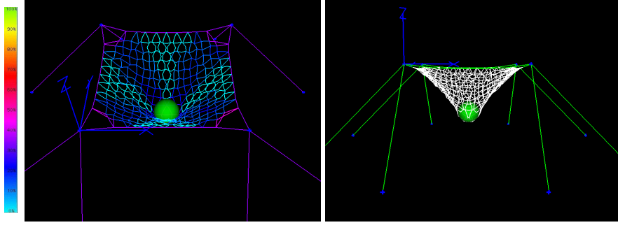
Figure 4: Simulation of single square, wire-ring net 3.90 m \times 3.90 m suspended on cables (Topview with degree of utilization of single elements)
