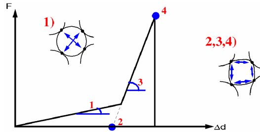
Figure 6: Modeling the net rings via single forces on their incidence nodes
