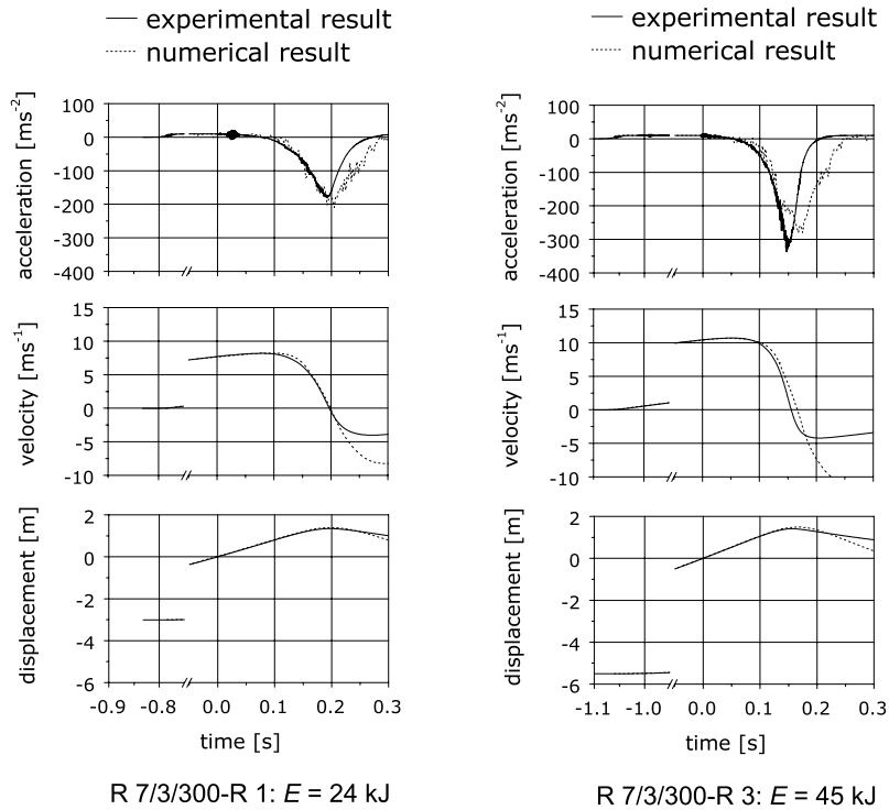
Figure 9: Single square, wire-ring net 3.90 \text{ m} \times 3.90 \text{ m} with blocked deformations: Data from the accelerometers in the boulder (vertical component)
