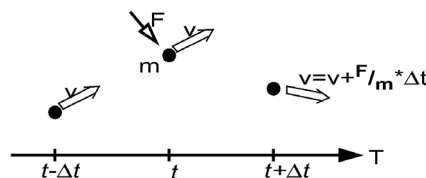
Figure 3: Functionality of the explicit algorithm
