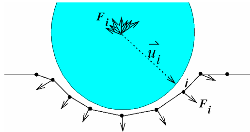
Figure 5: Contact computed with forces constraining the rock and the nodes
