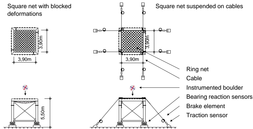
Figure 2: Plan and elevation of the field apparatus
