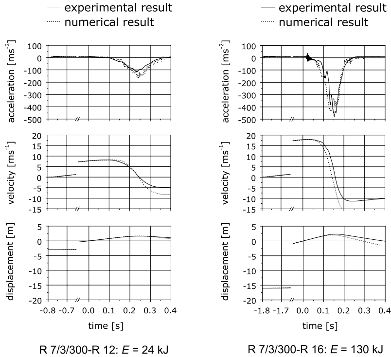
Figure 10: Single square, wire-ring net 3.90 \text{ m} \times 3.90 \text{ m} suspended on cables: Data from the accelerometers in the boulder (vertical component)
