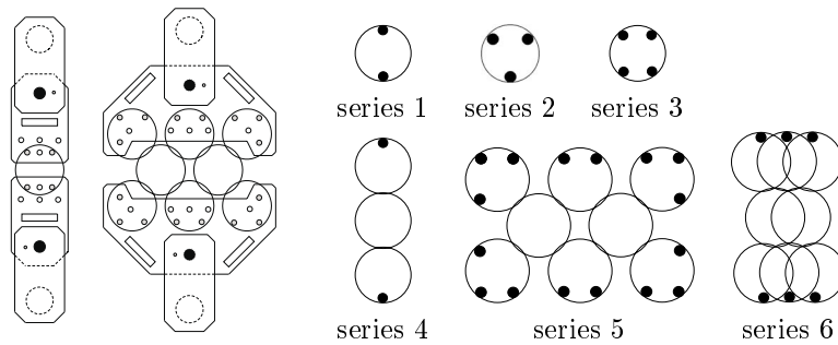
Figure 1: Quasi-static tensile tests with wire rings \varnothing 300 mm: Apparatus and overview of test series
