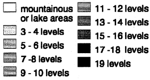
(a) Range of temperature within a mapping area (RTL); r = 0.58
